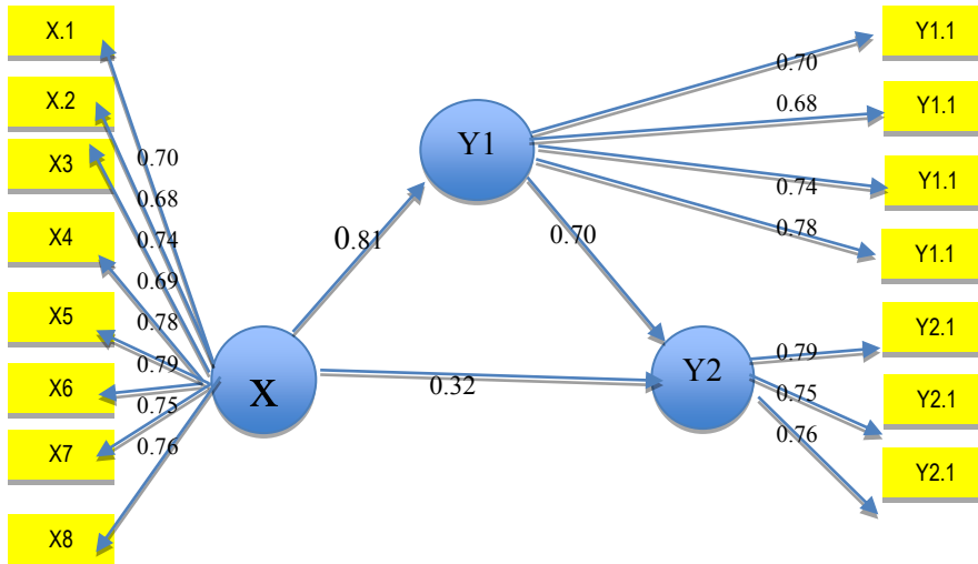
Figure 2. T-Test Diagram
